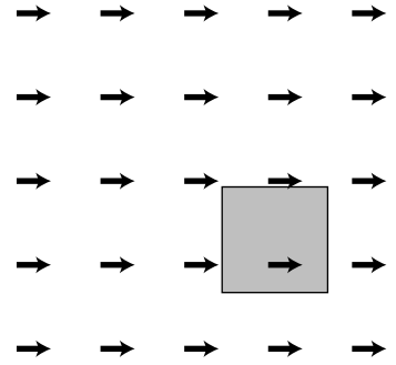
c / The field \hat{x} .
